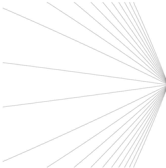
Level curves of \frac{|1-z|}{1-|z|} in the unit disk (top), and detail near z = 1 (bottom).
